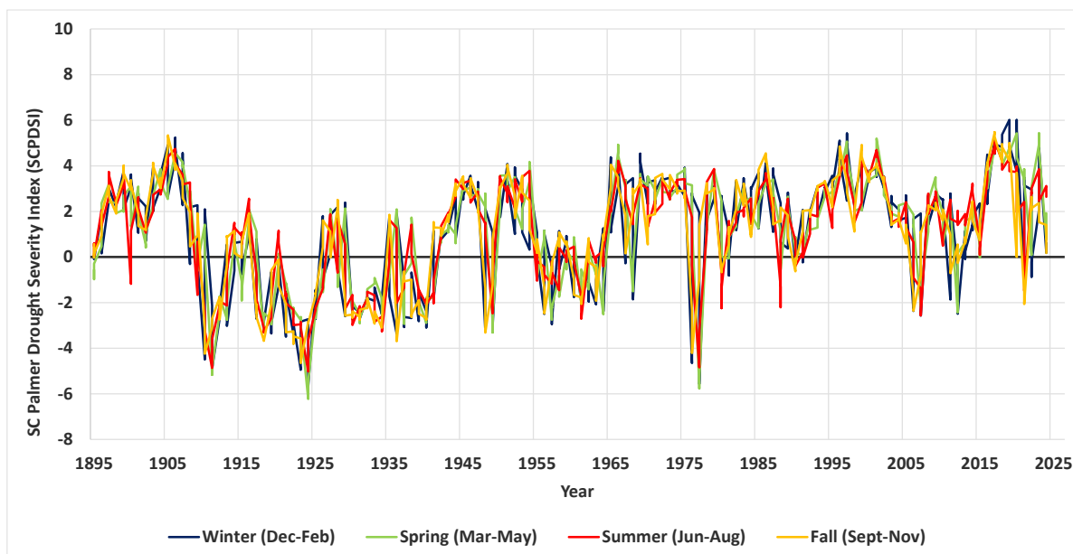
Figure 7-3 Historical Drought Severity for St. Louis County from 1895 to 2024
