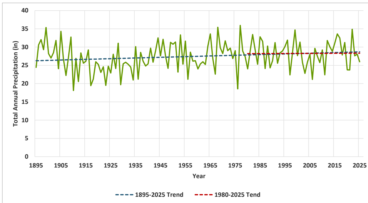
Figure 7-2 Historical Total Annual Precipitation (inches) for St. Louis County from 1895 to 2025 and 1980 to 2025
