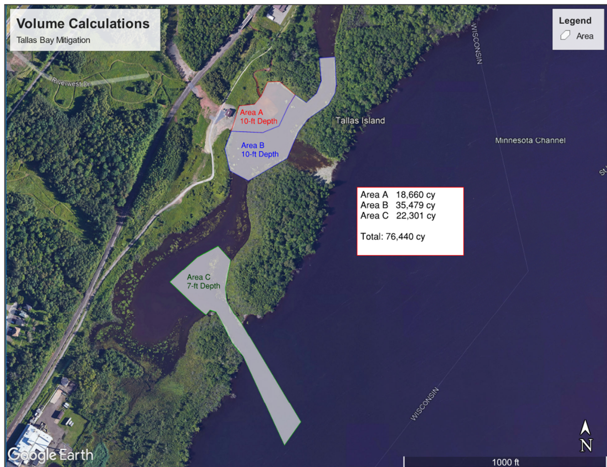
Figure 7. Preliminary Dredging Alternative
