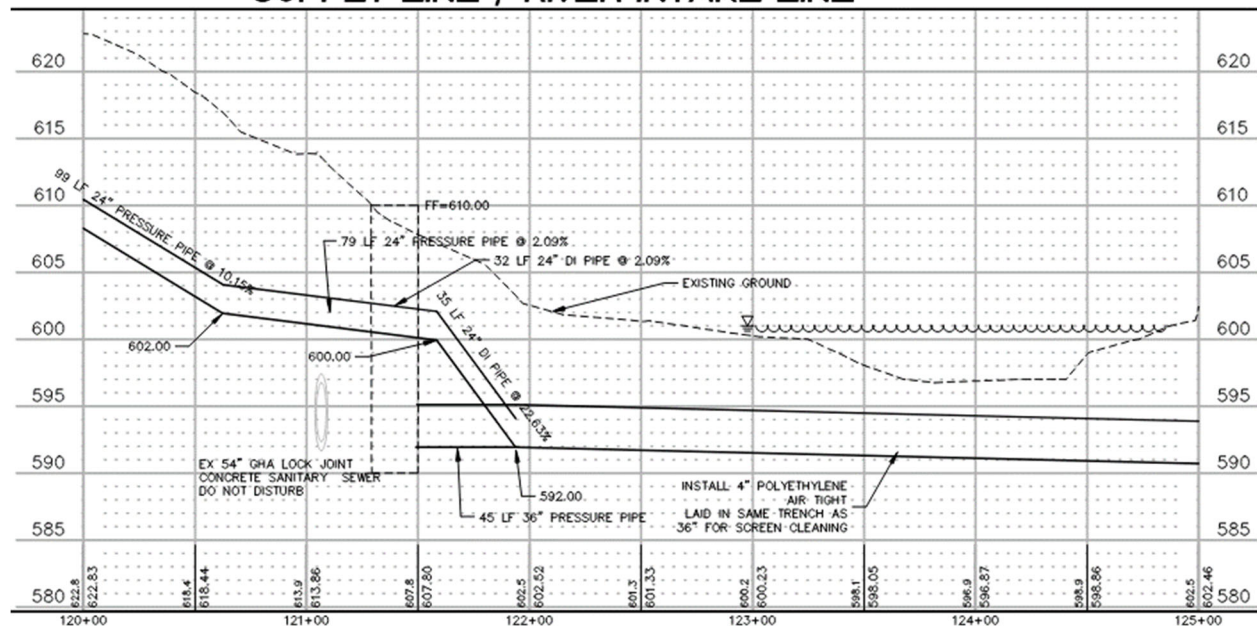
Figure 5. Plan and Section Drawings of Spirit Mountain Pipeline
