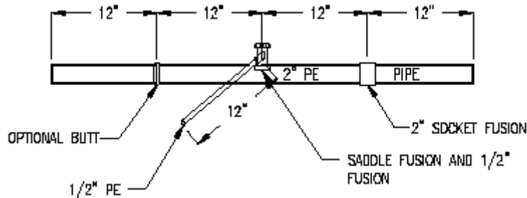
Figure 28-1 Fabricated Assembly for P.E. Fusion Qualification Test Part III
