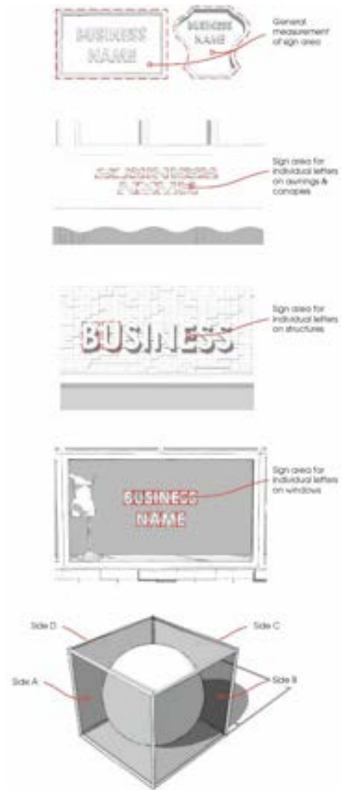
Figure 50-27.3-A: Sign dimension measurement methodology
