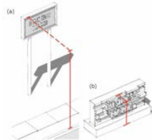
Figure 50-27.3-B: General dimension of sign height
