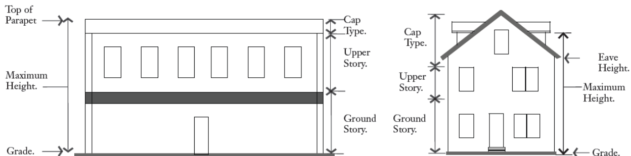
Figure 50-22.5-B: Measuring Height
