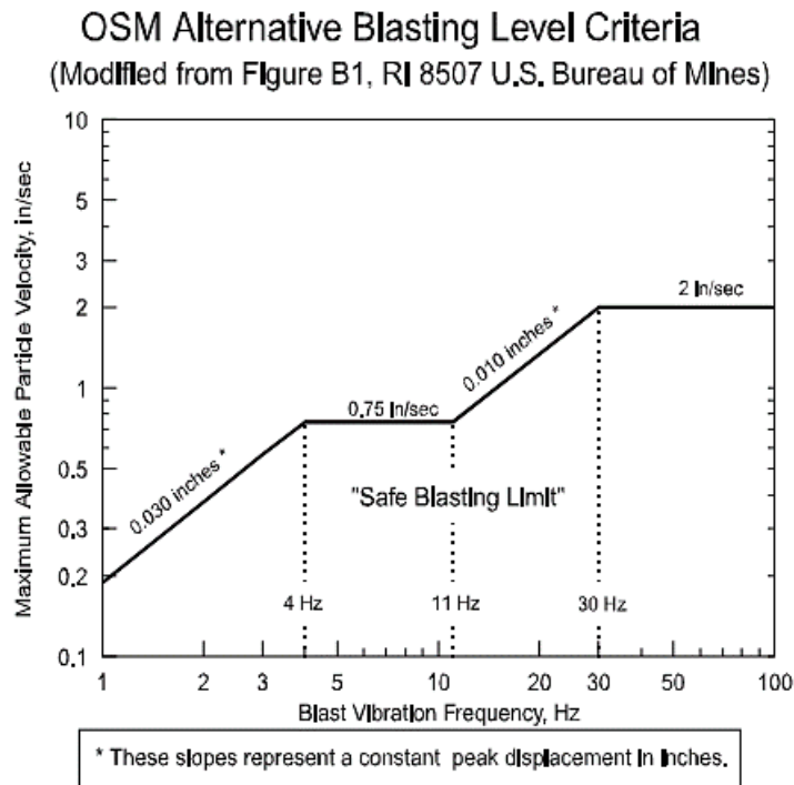
Figure 2015-1 OSM Alternative Blasting Level Criteria
