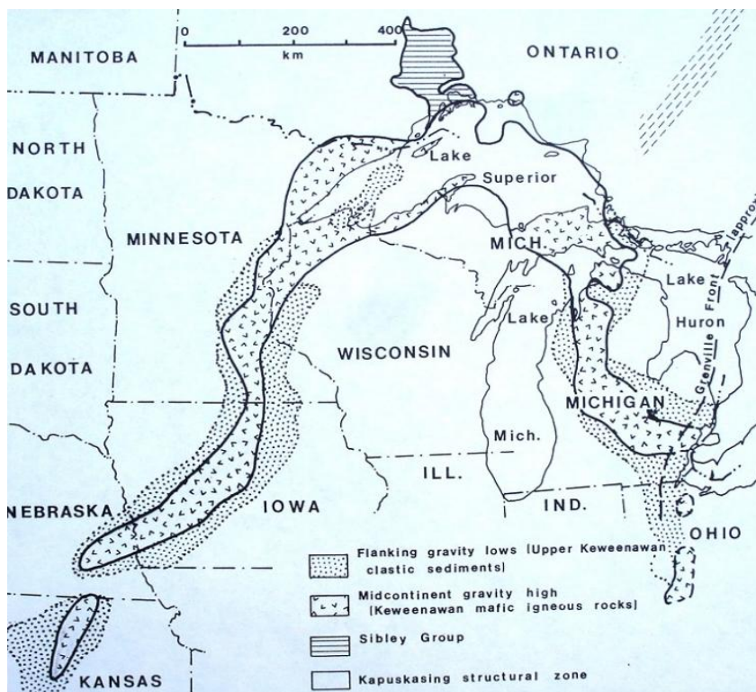
Figure 7: Map of mid-continental rift.
