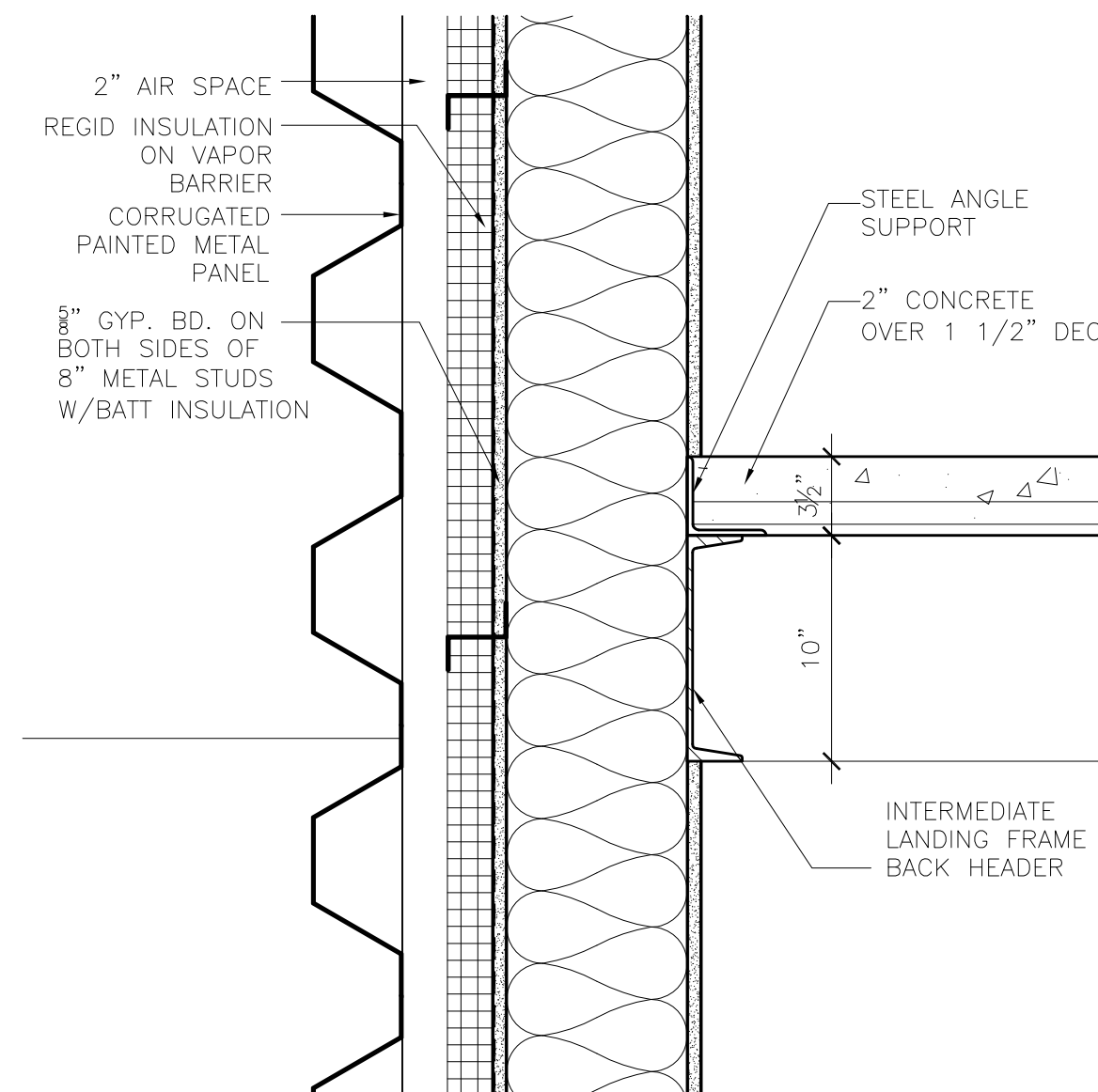
3 LANDING TO WALL DEDETAIL 1 1/2" = 1'-0"
