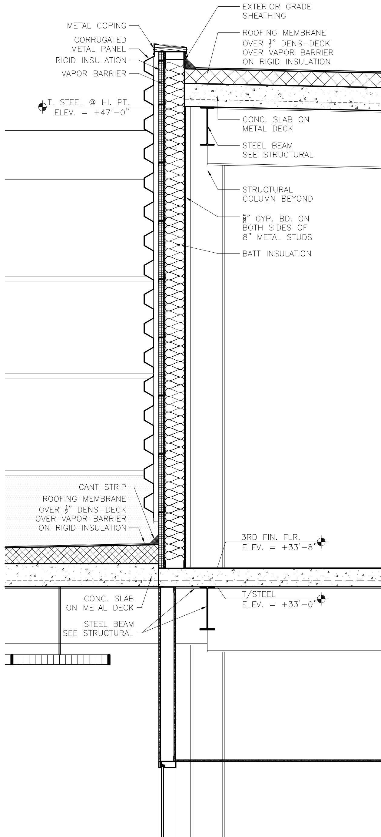
3 WALL SECTION @ CORE WALL 1/2" = 1'-0"
