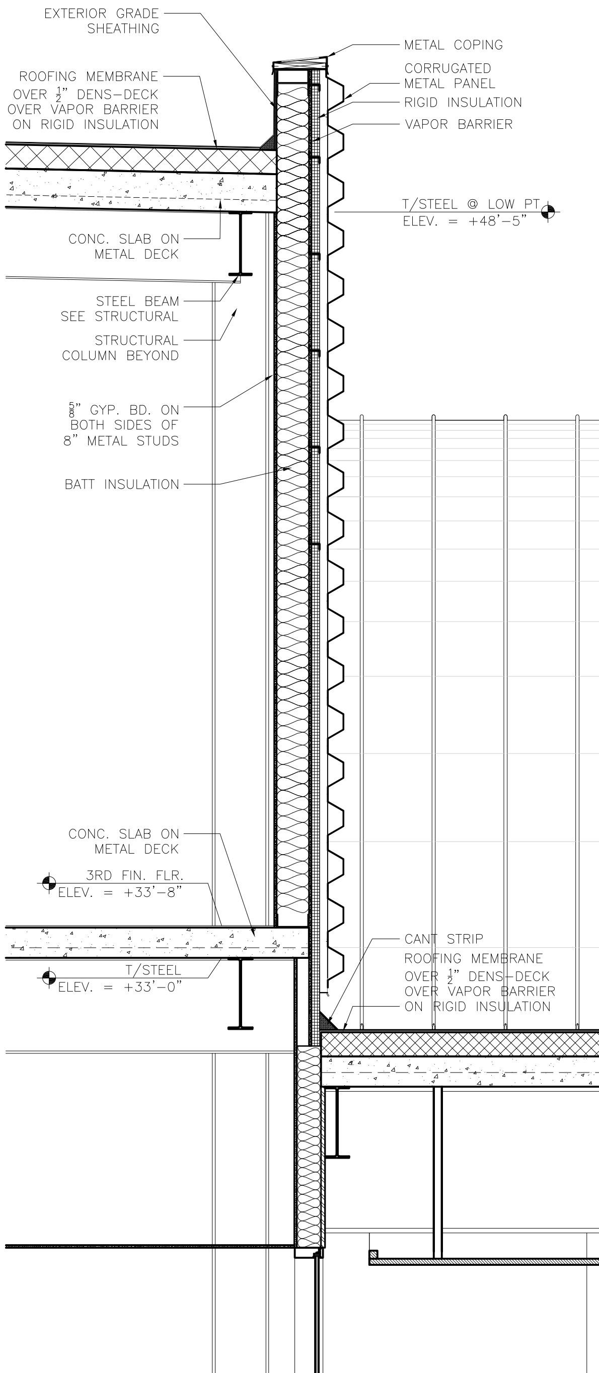
2 WALL SECTION @ CORE WALL 1/2" = 1'-0"
