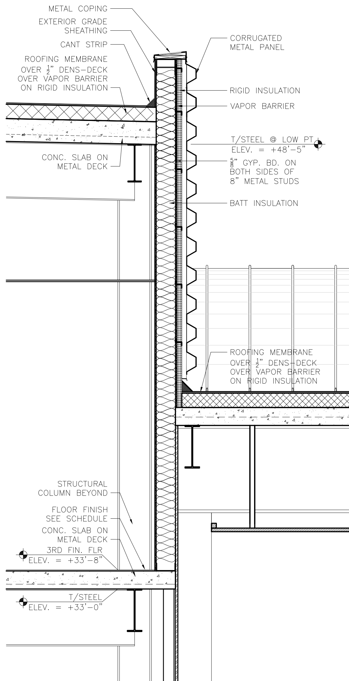
1 WALL SECTION @ CORE WALL 1/2" = 1'-0"
