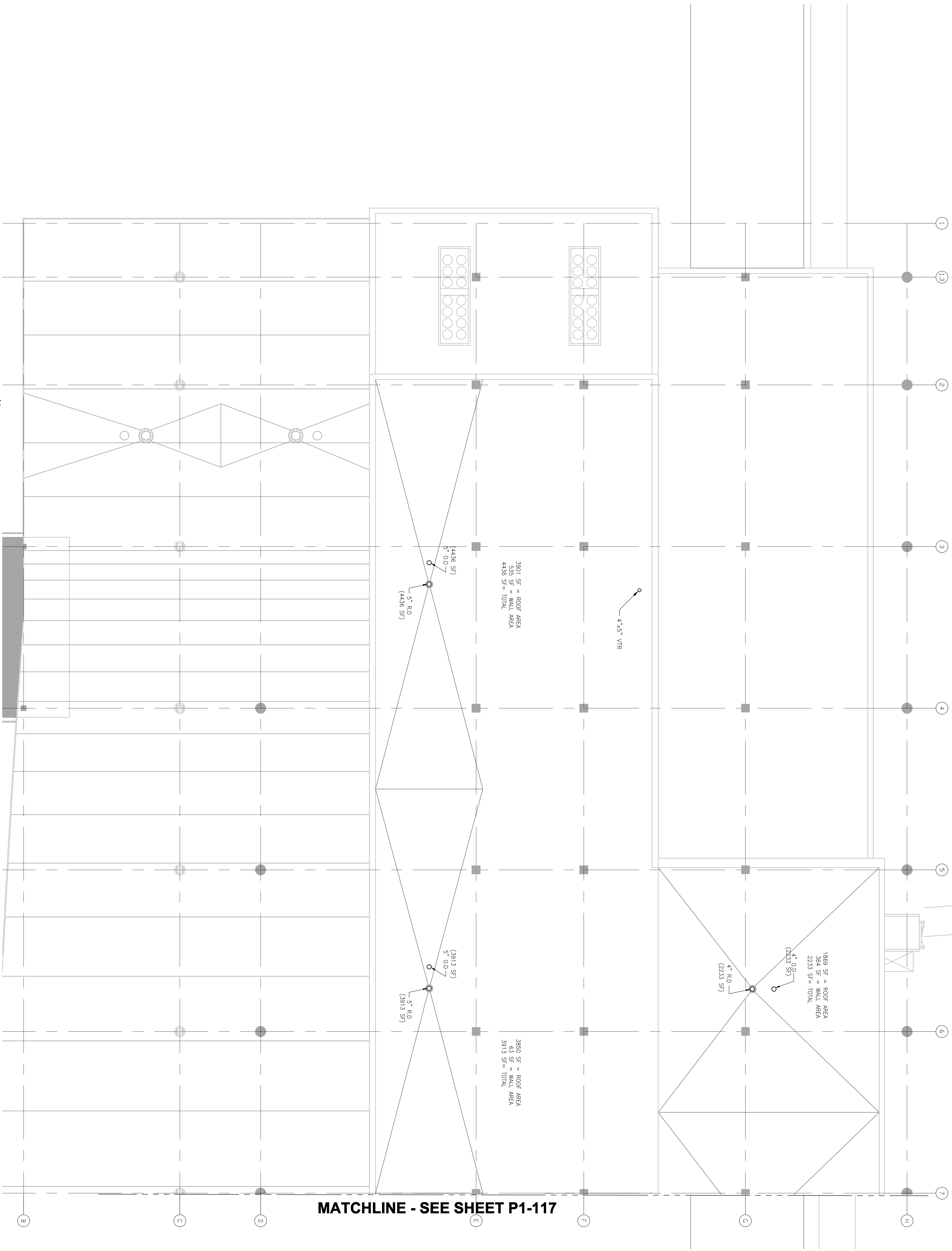
1 1/8"=1'-0" ENLARGED ROOF LEVEL PLAN - AREA A
