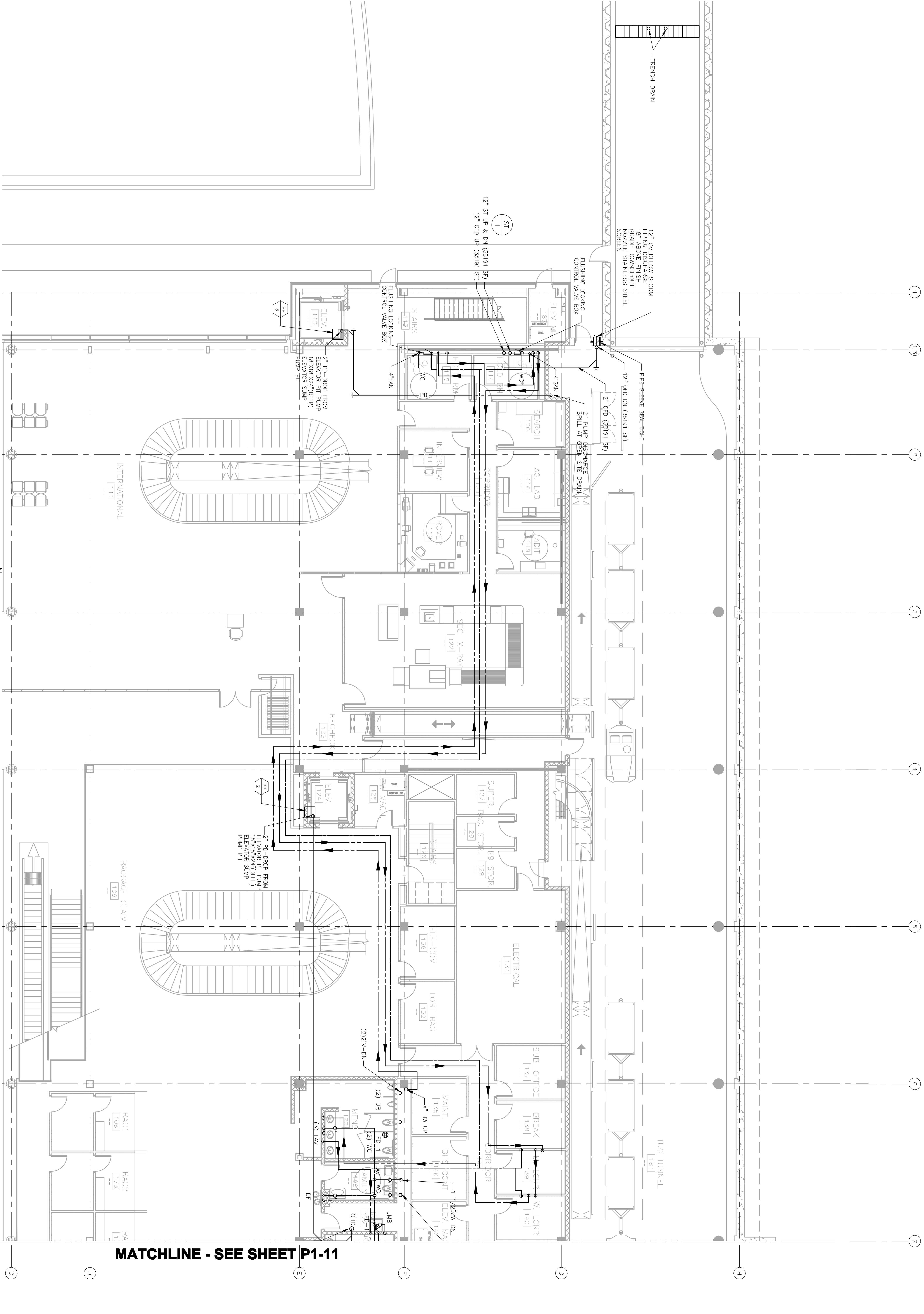
1 ENLARGED FIRST LEVEL FLOOR PLAN - AREA A 1/8" = 1'-0"
