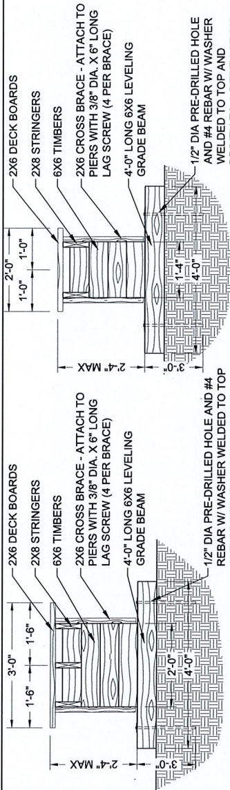
36" WIDE BOARDWALK
