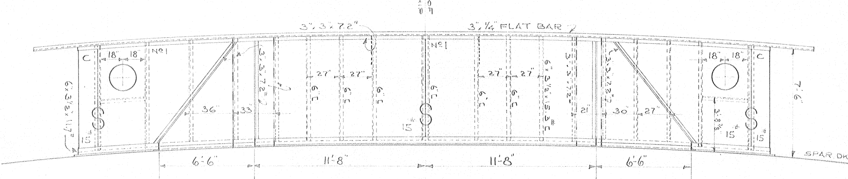
ELEVATION OF FORWARD END LOOKING AFT 5'-3 1/8\"/>
