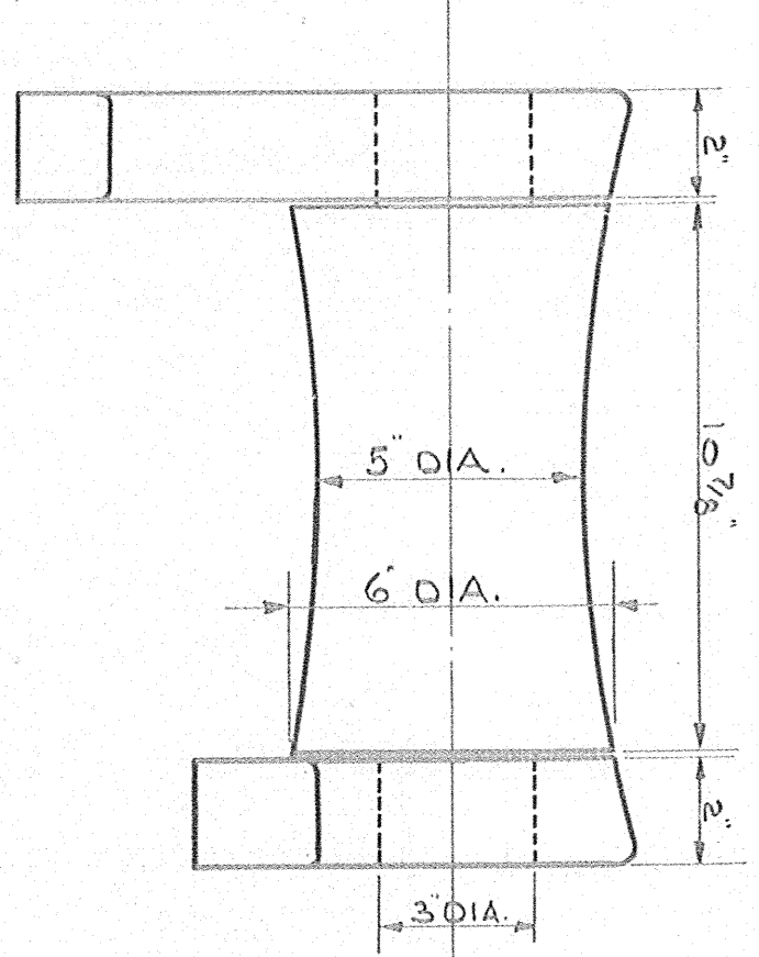
C.R. STEEL ROLLER CAST STEEL BRACKETS SCALE = 3/4\"/>
