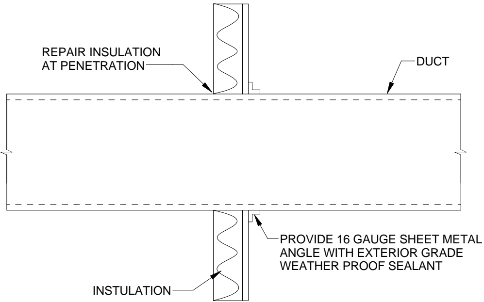
3 DUCT PENETRATION DETAIL ME3 NO SCALE
