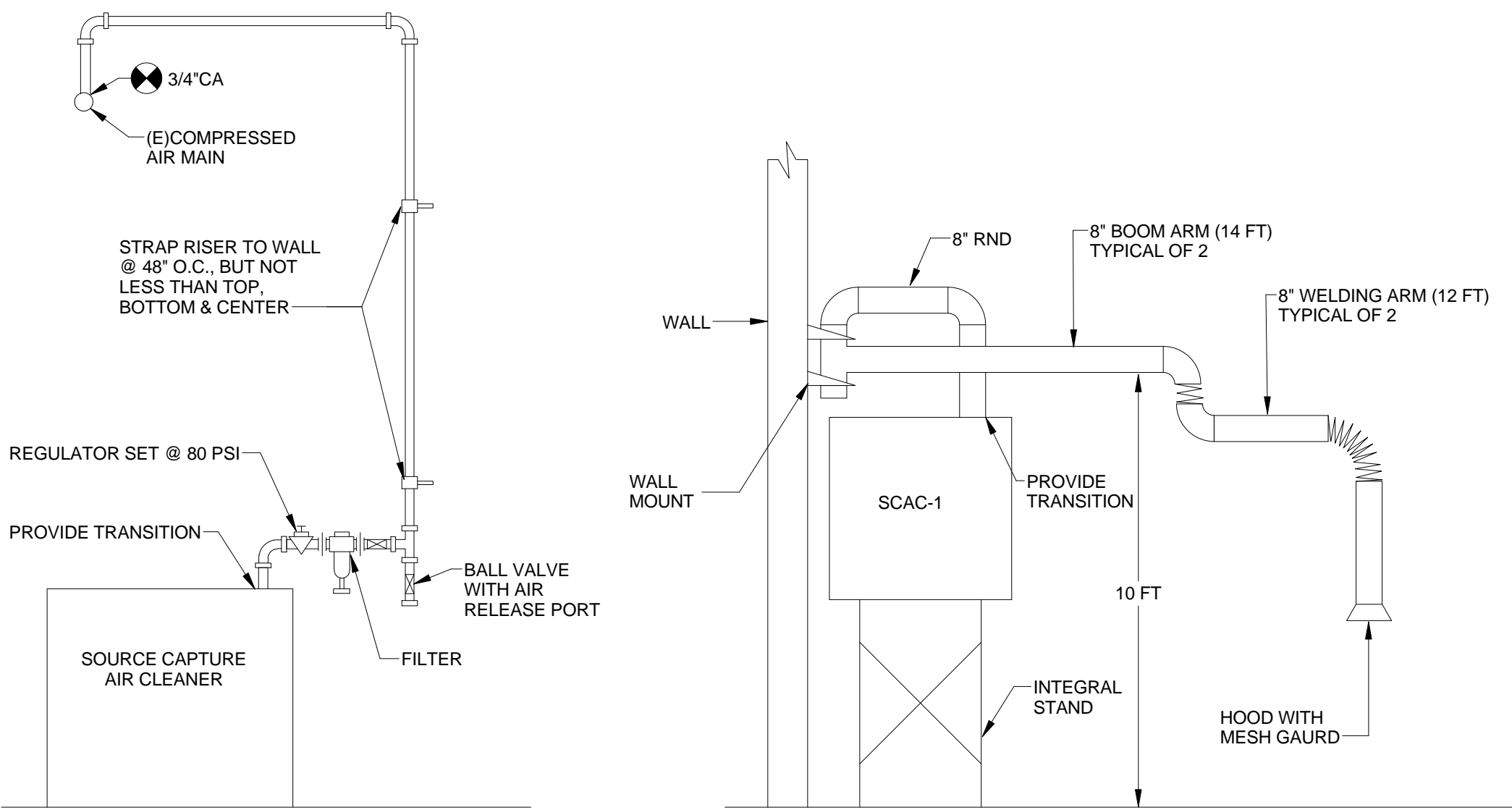
4 COMPRESSED AIR CONNECTION DETAIL ME3 NO SCALE
