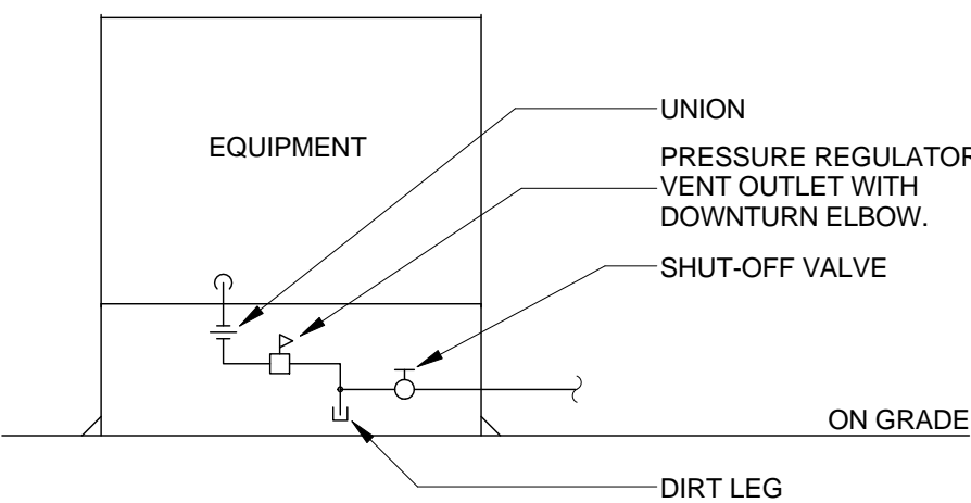
5 GAS PIPING CONNECTION DETAIL ME3 NO SCALE
