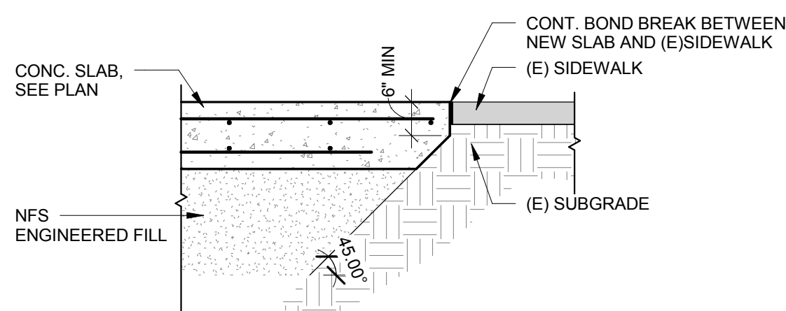
8 SLAB EDGE AT SIDEWALK S501 1/2" = 1'-0"
