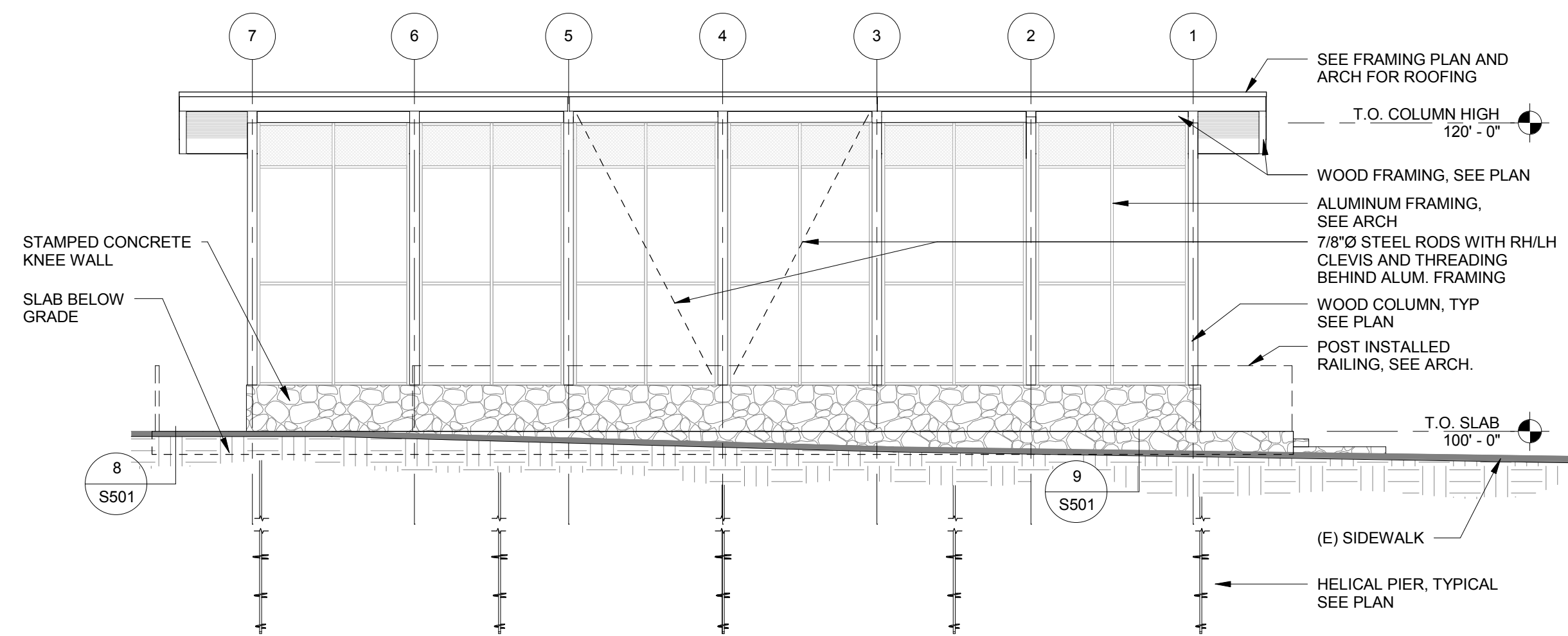
3 NORTH ELEVATION - STRUCTURAL S101 1/8" = 1'-0"
