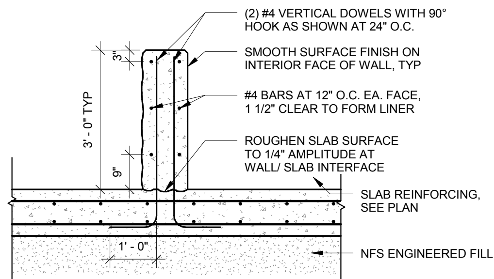
5 KNEE WALL TO SLAB CONNECTION S501 1/2" = 1'-0"
