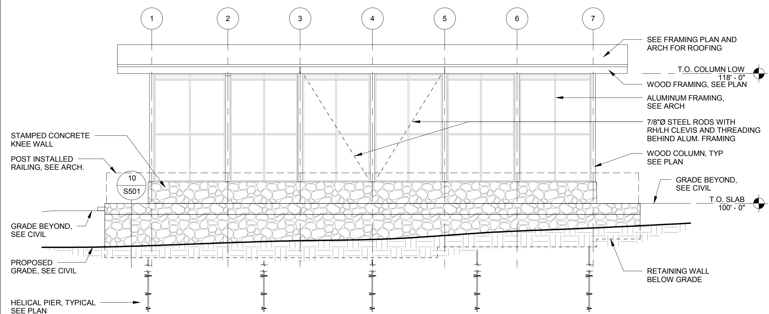
5 SOUTH ELEVATION - STRUCTURAL S101 1/8" = 1'-0"
