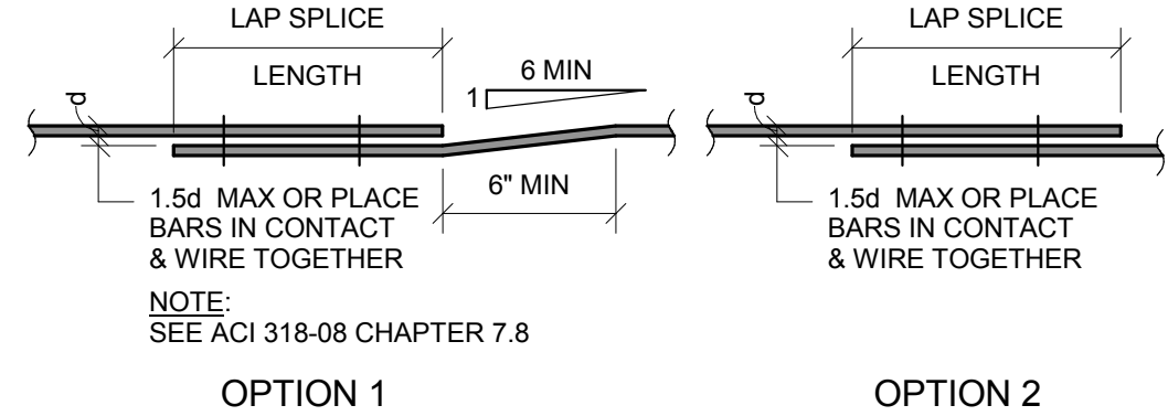
1 TYPICAL CONCRETE SPLICE REINFORCING DETAIL S501 3/4" = 1'-0"
