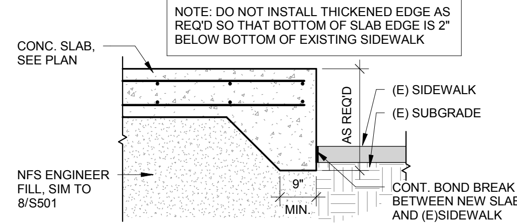
9 THICKENED SLAB EDGE AT SIDEWALK S501 1/2" = 1'-0"
