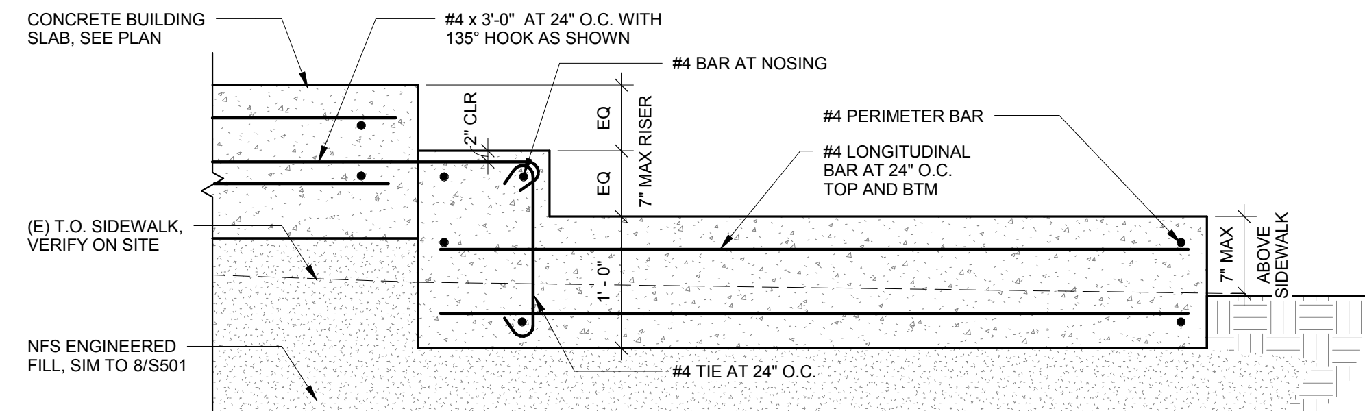
11 CONCRETE STAIR SECTION S501 1" = 1'-0"
