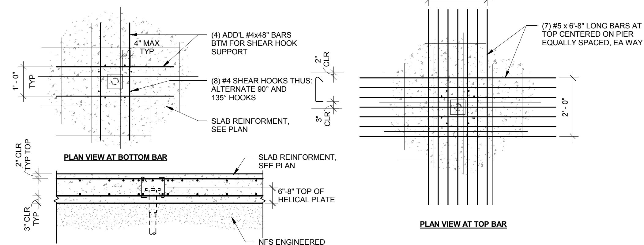
7 PILE CAP INTO SLAB S501 1/2" = 1'-0"
