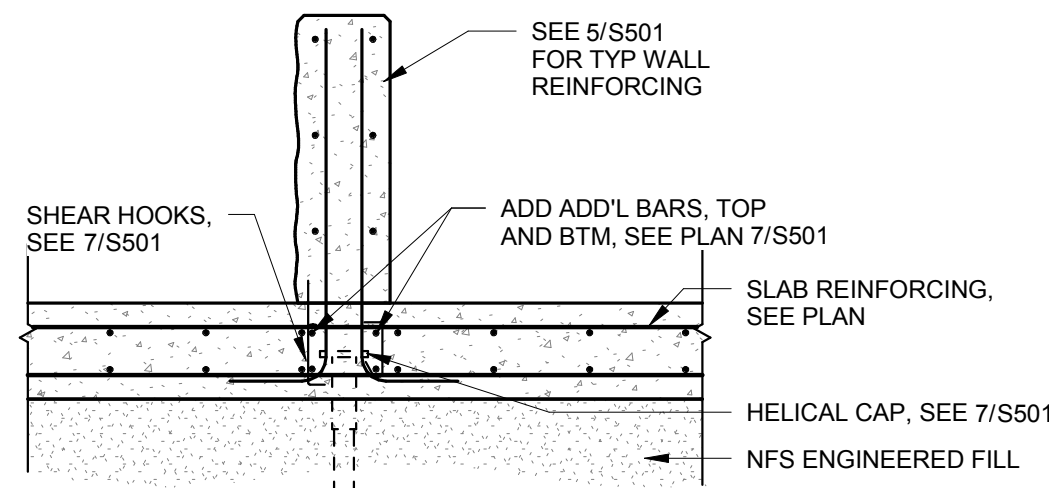
6 KNEE WALL TO SLAB CONNECTION AT PILE S501 1/2" = 1'-0"
