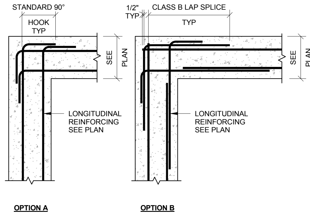
2 TYPICAL CONCRETE CORNER DOUBLE MAT REINFORCING S501 3/4" = 1'-0"
