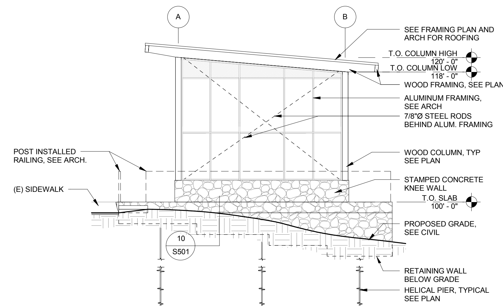
4 WEST ELEVATION - STRUCTURAL S101 1/8" = 1'-0"
