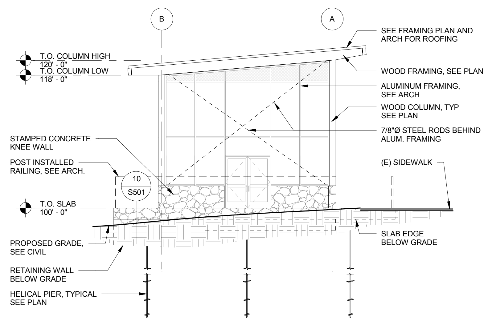
6 EAST ELEVATION - STRUCTURAL S101 1/8" = 1'-0"
