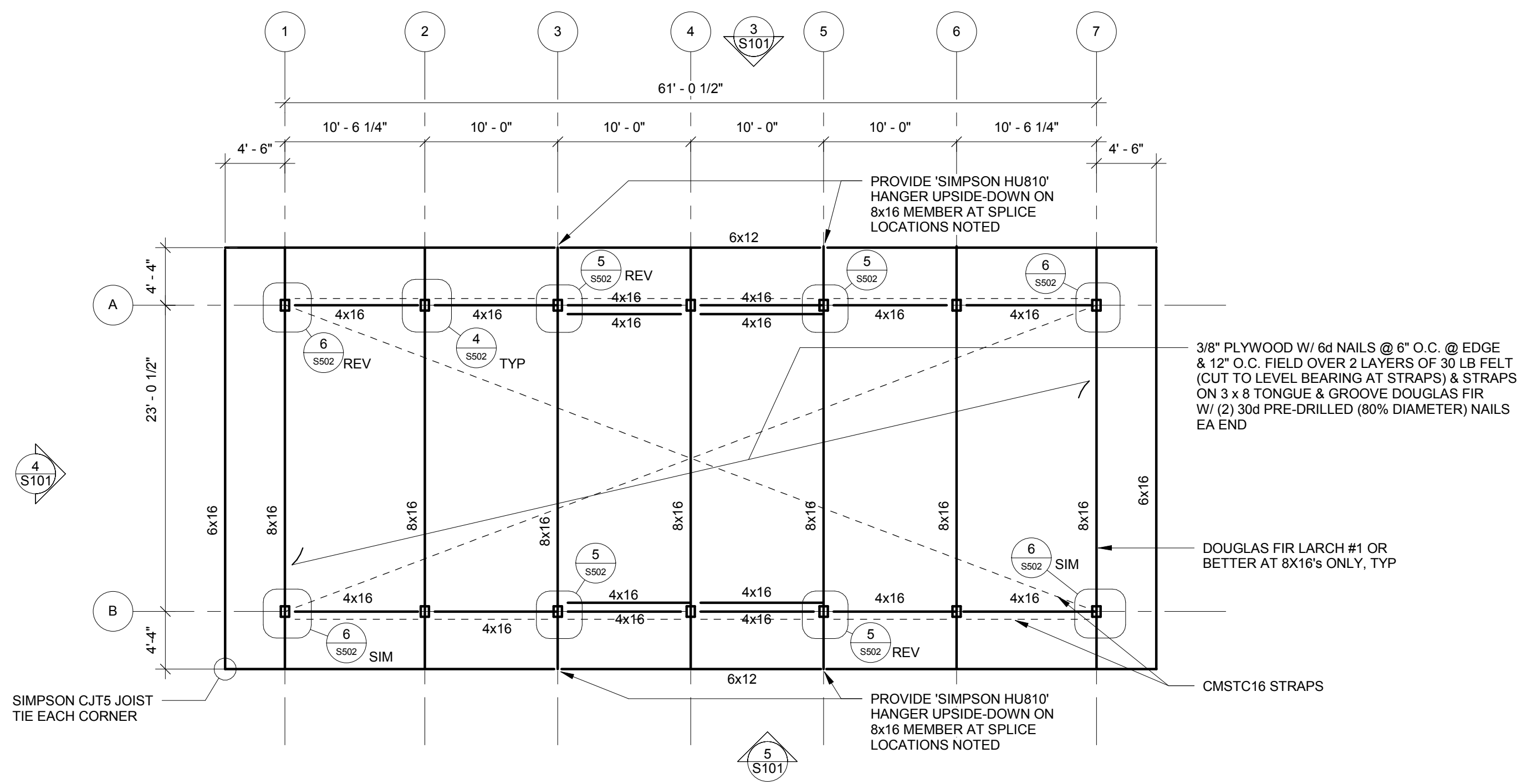
2 FRAMING PLAN S101 1/8" = 1'-0"
