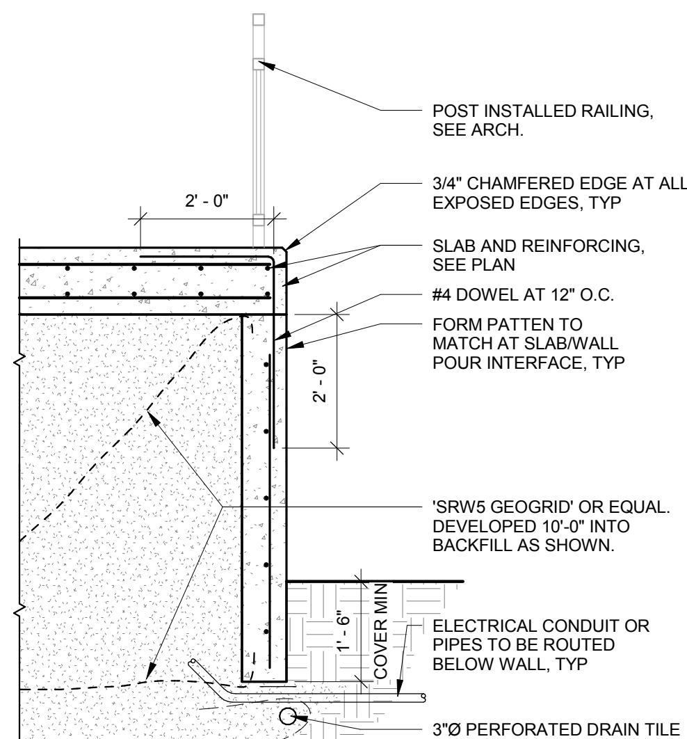
10 SLAB EDGE WITH RETAINING WALL S501 1/2" = 1'-0"
