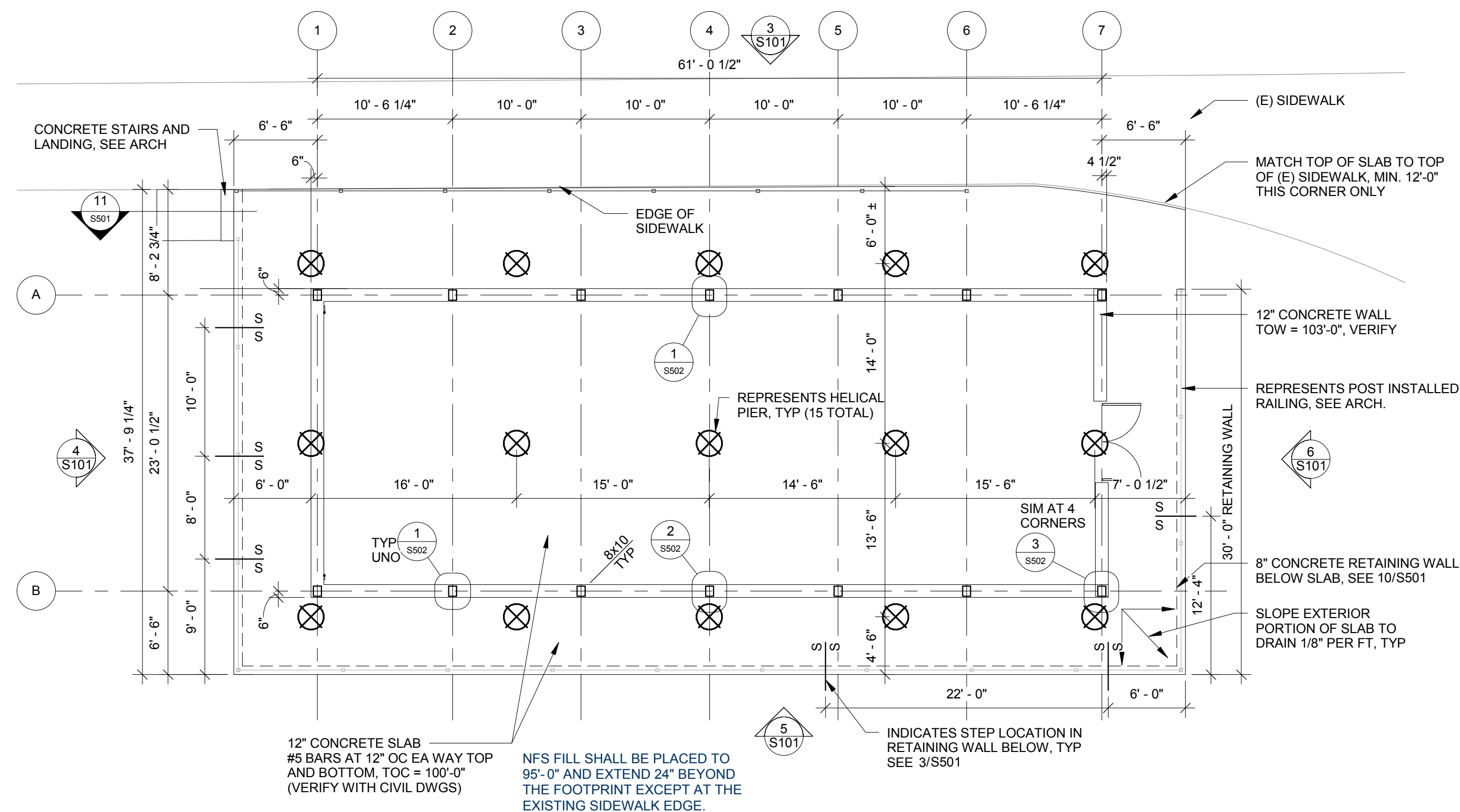
1 FOUNDATION PLAN S101 1/8" = 1'-0"
