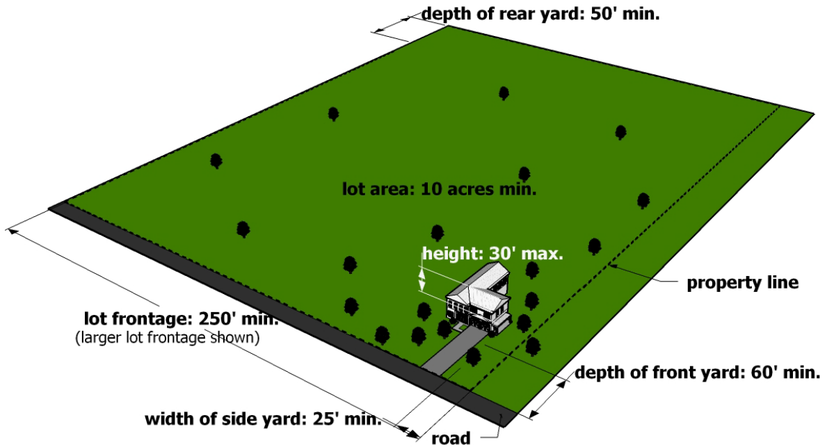
R-C Example Lot Layout
