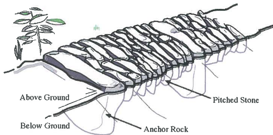
Figure 5: Tread Rock Armoring
