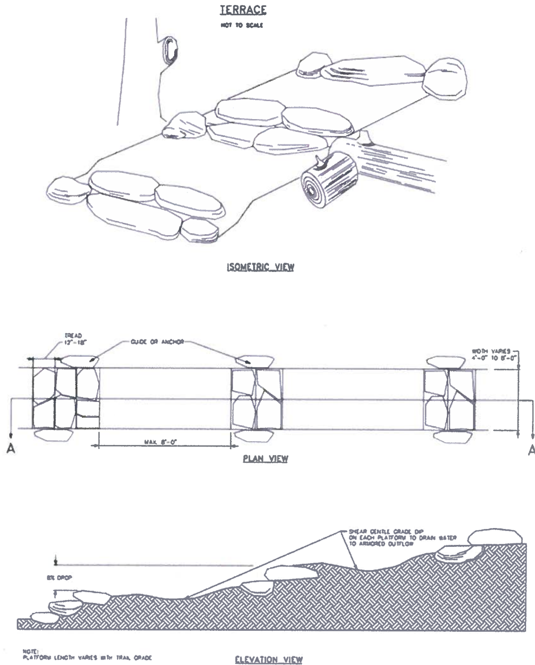
Figure 8: Terrace
