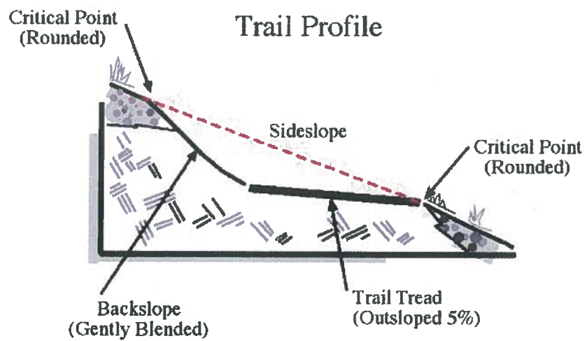
Figure 3: Full Bench Trail
