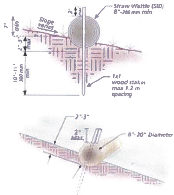
Figure 13: Straw Wattle Installation
