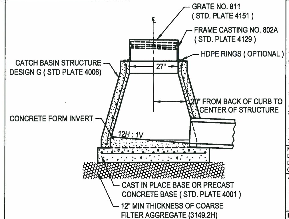
6 FABRIC WRAPPED CATCH BASIN CASTING C2.0 NOT TO SCALE
