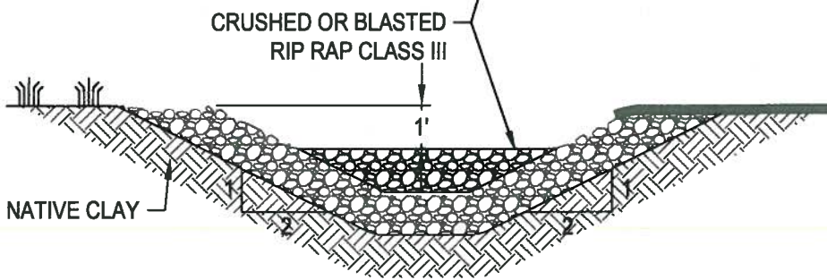
PROFILE VIEW
