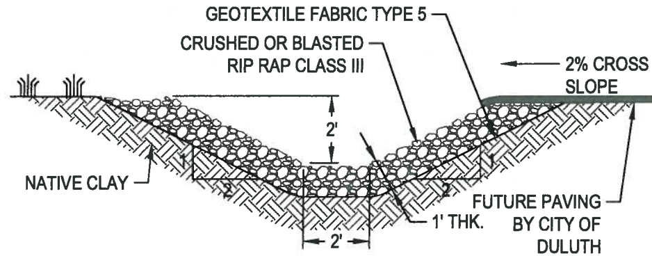
1 TYPE 1 DITCH SECTION C2.0 NOT TO SCALE
