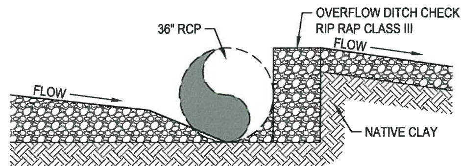
PROFILE VIEW
