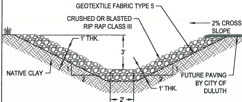
1 TYPE 1 DITCH SECTION C2.0 NOT TO SCALE
