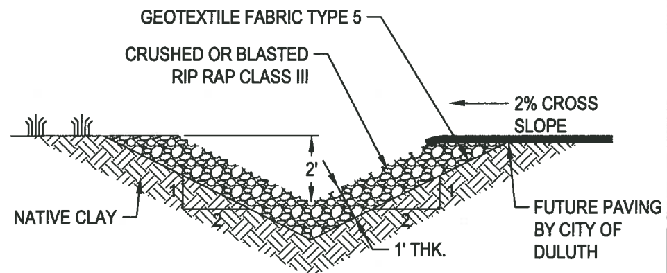
3 TYPE 3 DITCH SECTION C2.0 NOT TO SCALE
