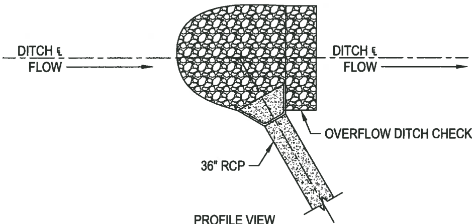
PROFILE VIEW
