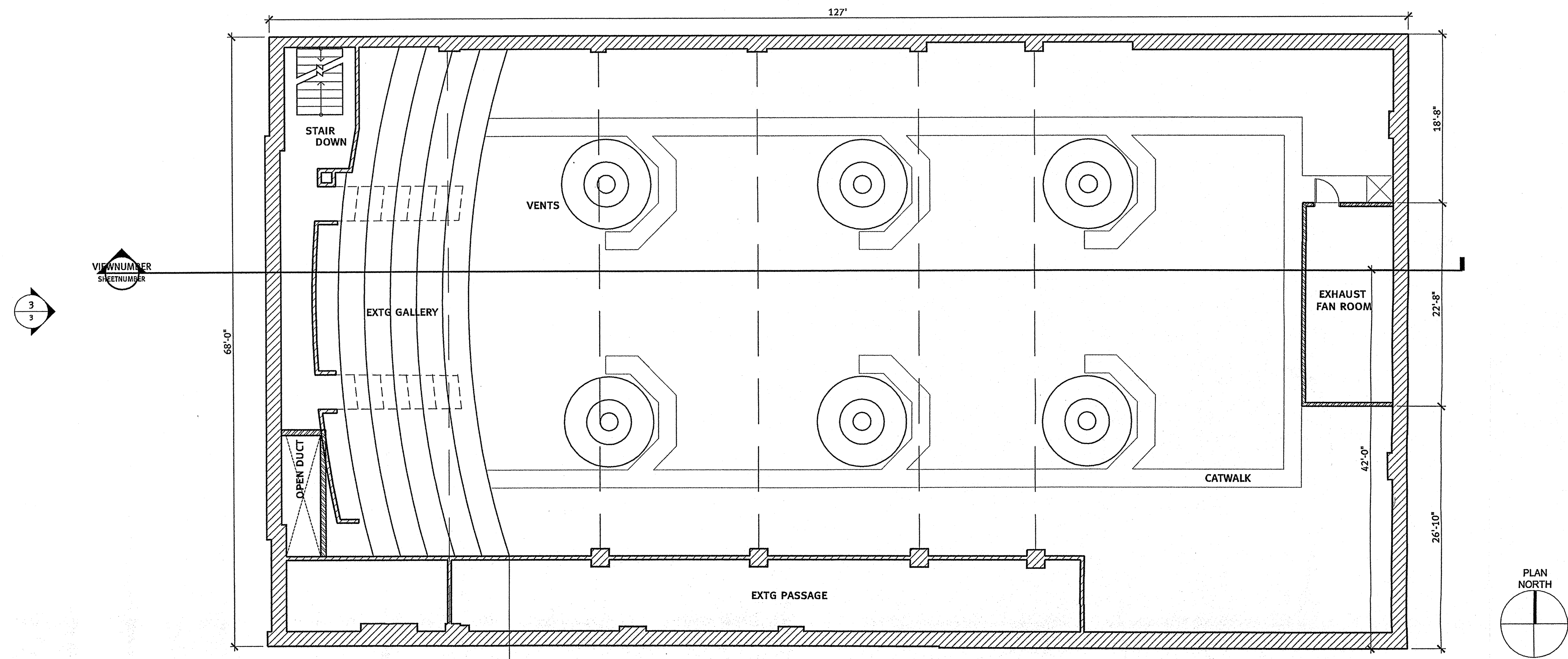
1 ATTIC SPACE 2-15-07 1/8"=1'-0"
